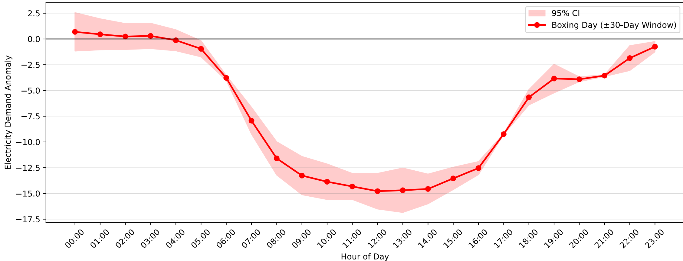
Castle Cove Demand Anomaly: Boxing Day (2010-2011, \pm 30 -Day Window)
