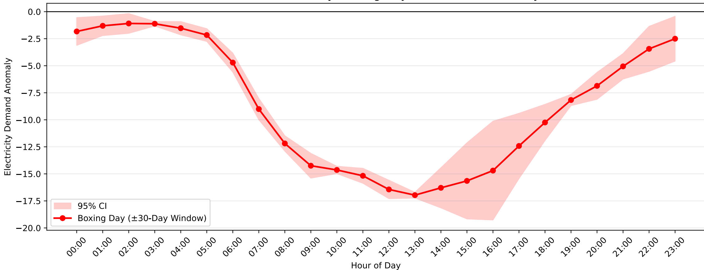
Castle Cove Demand Anomaly: Boxing Day (2012-2013, \pm 30 -Day Window)
