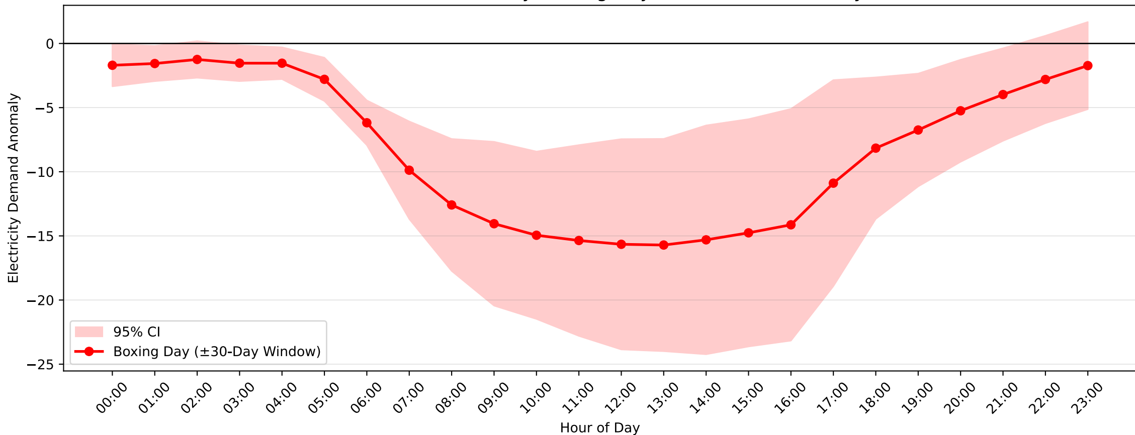
Castle Cove Demand Anomaly: Boxing Day (2007-2008, \pm 30 -Day Window)
