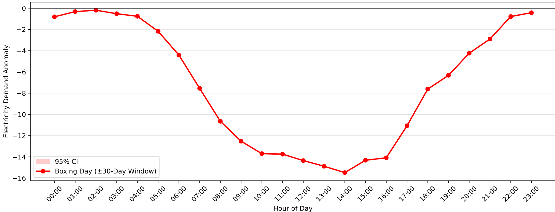
Castle Cove Demand Anomaly: Boxing Day (2004-2005, \pm 30 -Day Window)
