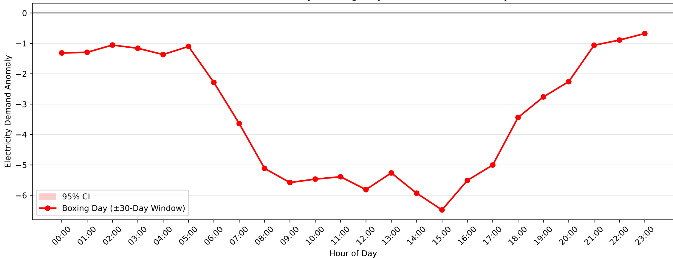
Castle Cove Demand Anomaly: Boxing Day (2016–2017, \pm 30 -Day Window)
