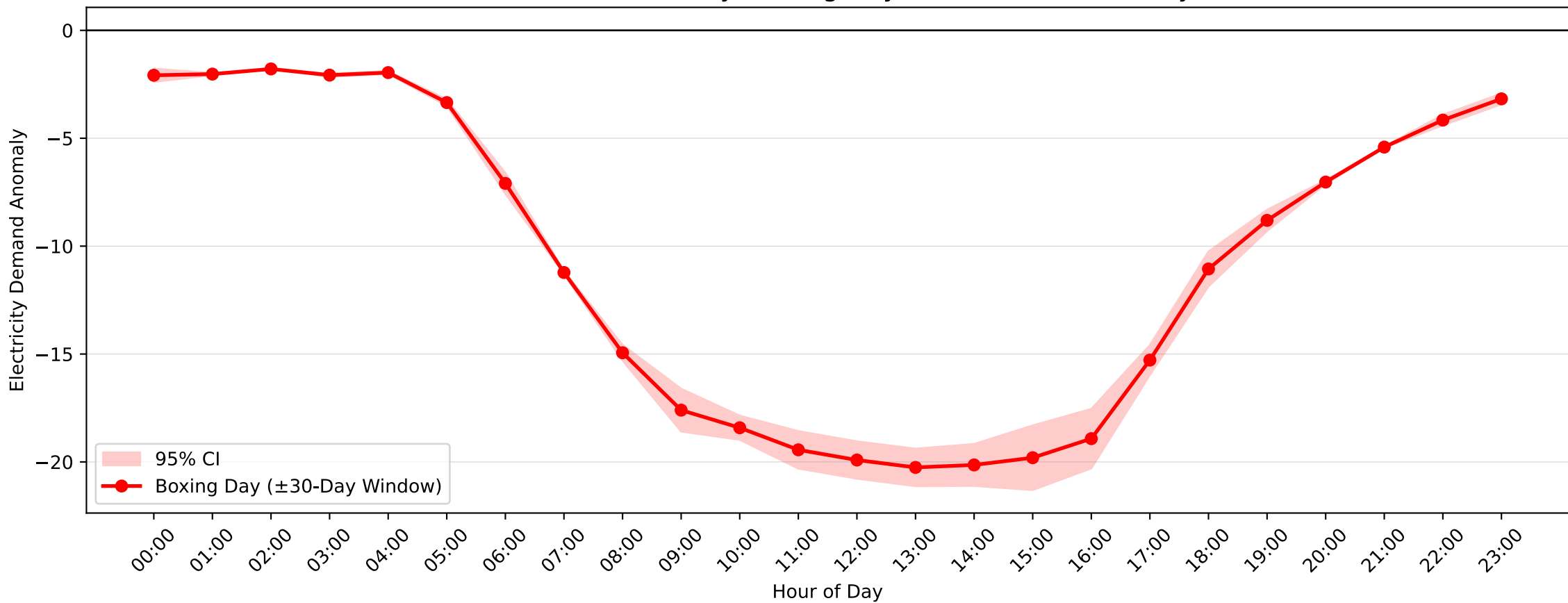
Castle Cove Demand Anomaly: Boxing Day (2006–2007, \pm 30 -Day Window)
