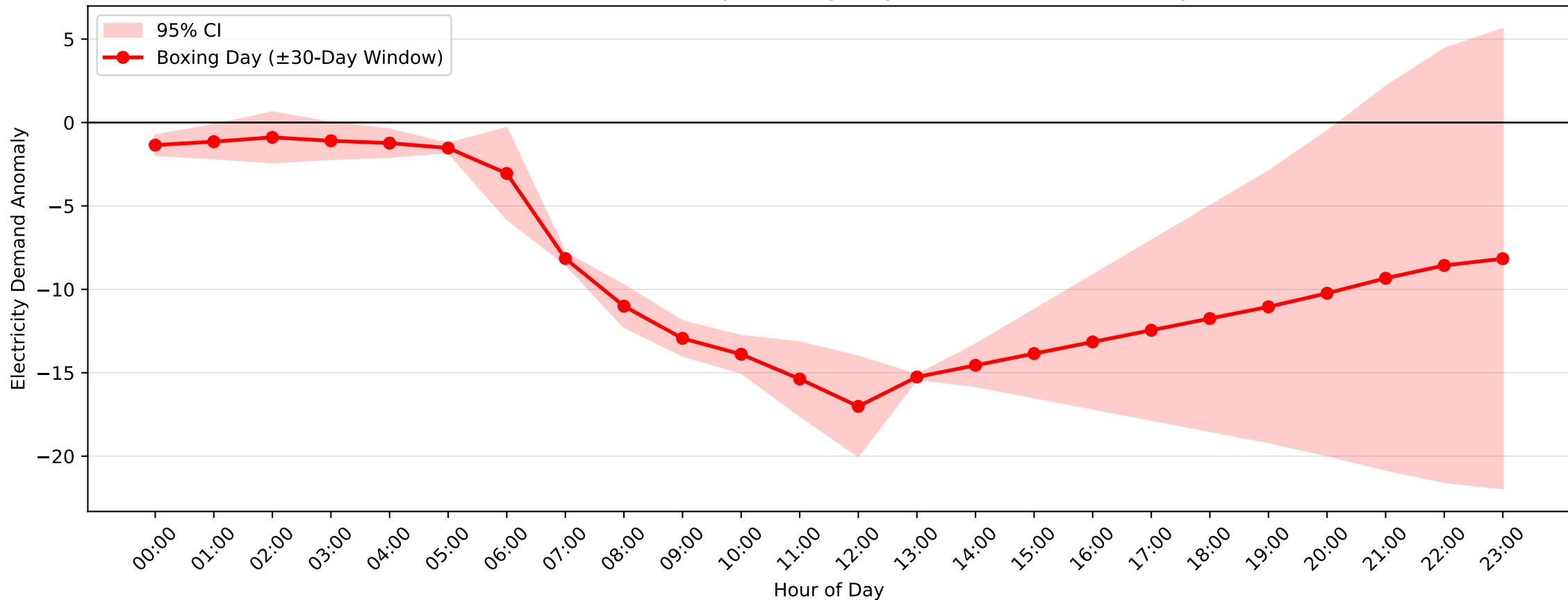
Castle Cove Demand Anomaly: Boxing Day (2013-2014, \pm 30 -Day Window)
