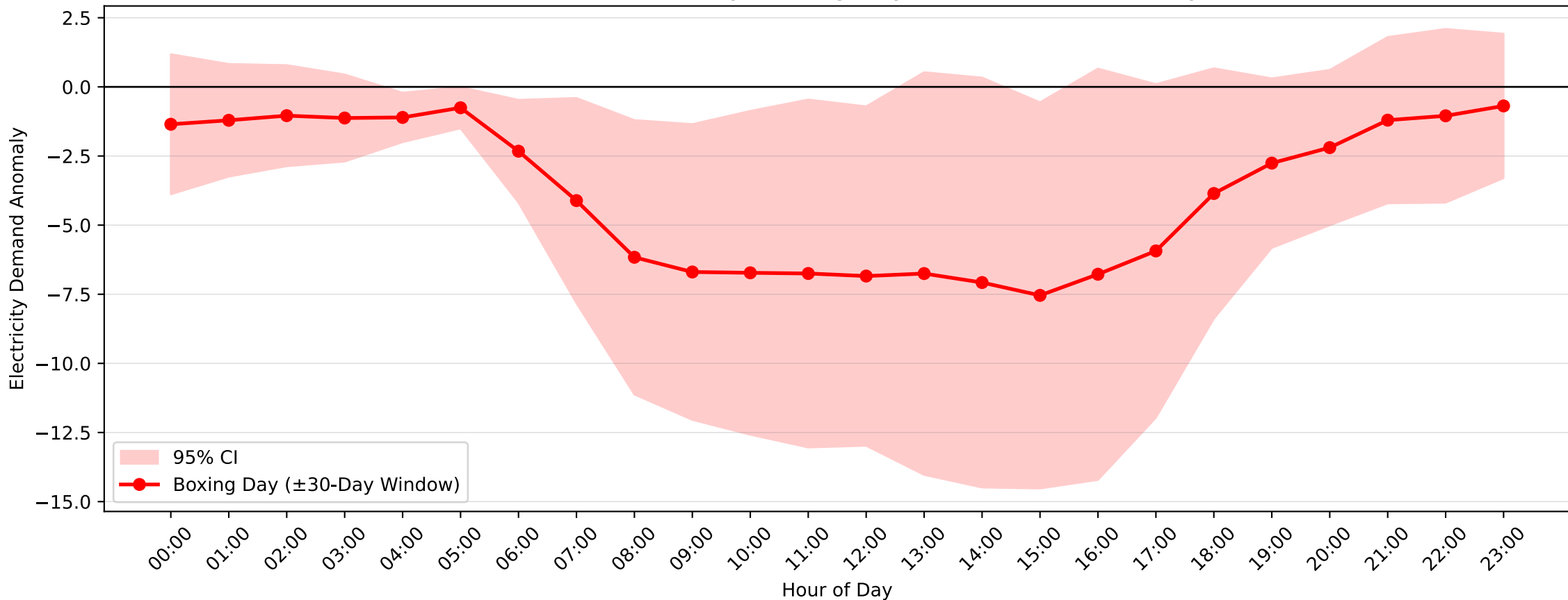
Castle Cove Demand Anomaly: Boxing Day (2015–2016, \pm 30 -Day Window)
