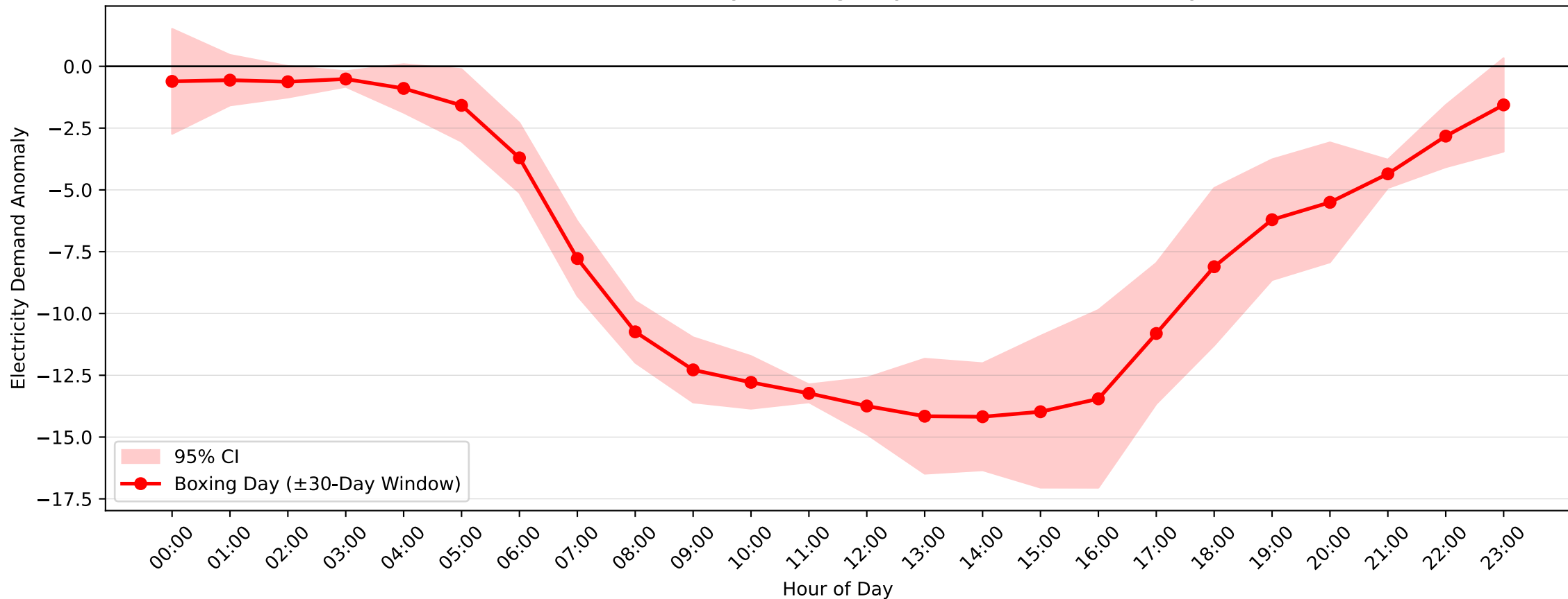
Castle Cove Demand Anomaly: Boxing Day (2011-2012, \pm 30 -Day Window)
