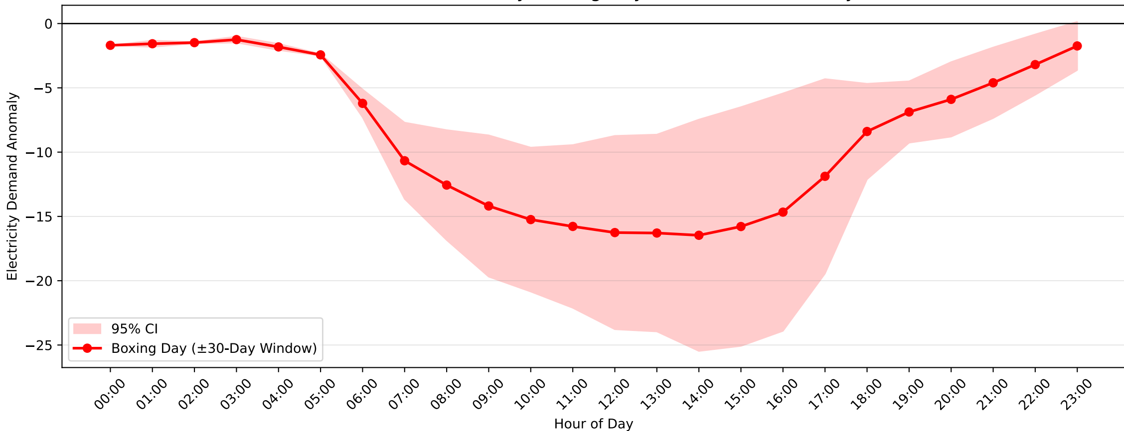
Castle Cove Demand Anomaly: Boxing Day (2008–2009, \pm 30 -Day Window)
