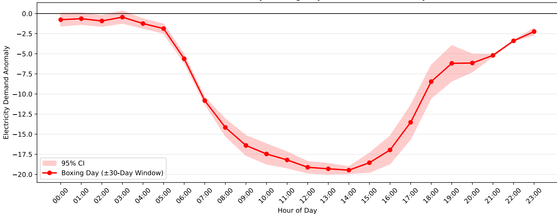
Castle Cove Demand Anomaly: Boxing Day (2009–2010, \pm 30 -Day Window)
