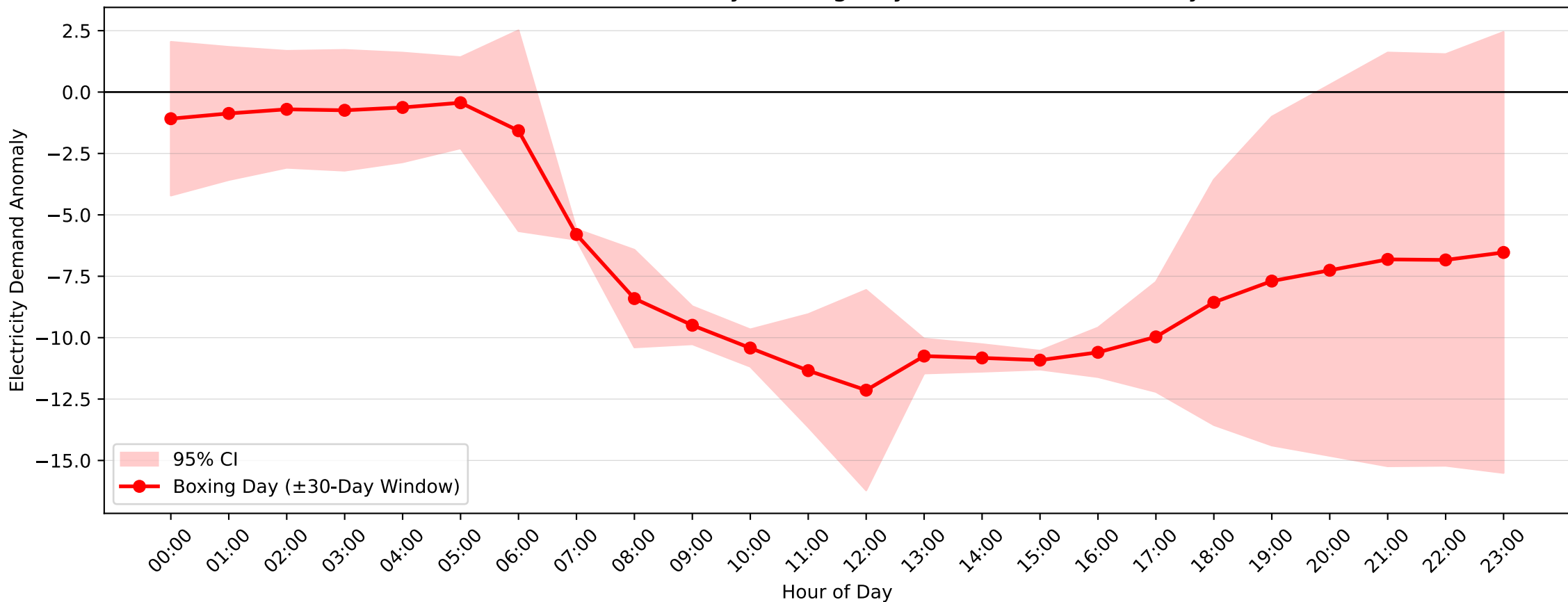
Castle Cove Demand Anomaly: Boxing Day (2014-2015, \pm 30 -Day Window)
