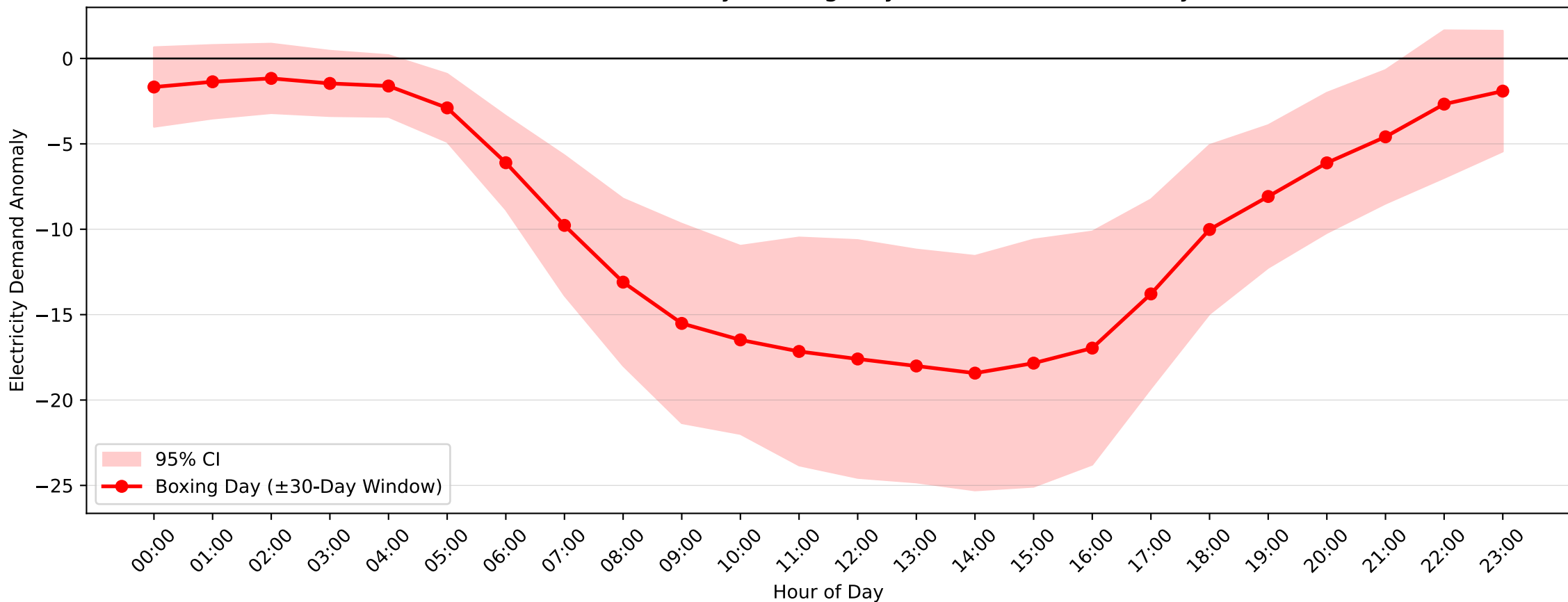
Castle Cove Demand Anomaly: Boxing Day (2005–2006, \pm 30 -Day Window)
